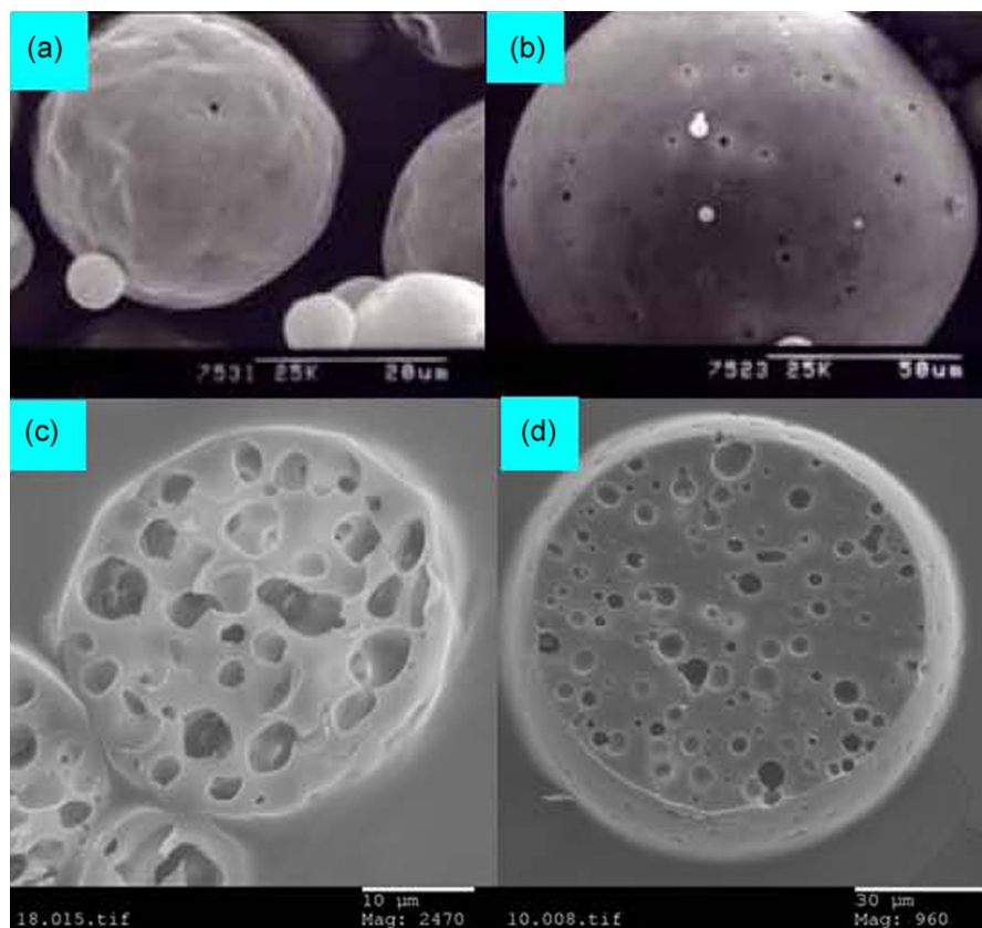
Fig. 3. Surface and internal morphology of microspheres prepared with 8% PLGA (a, c) and 32% PLGA (b, d).
