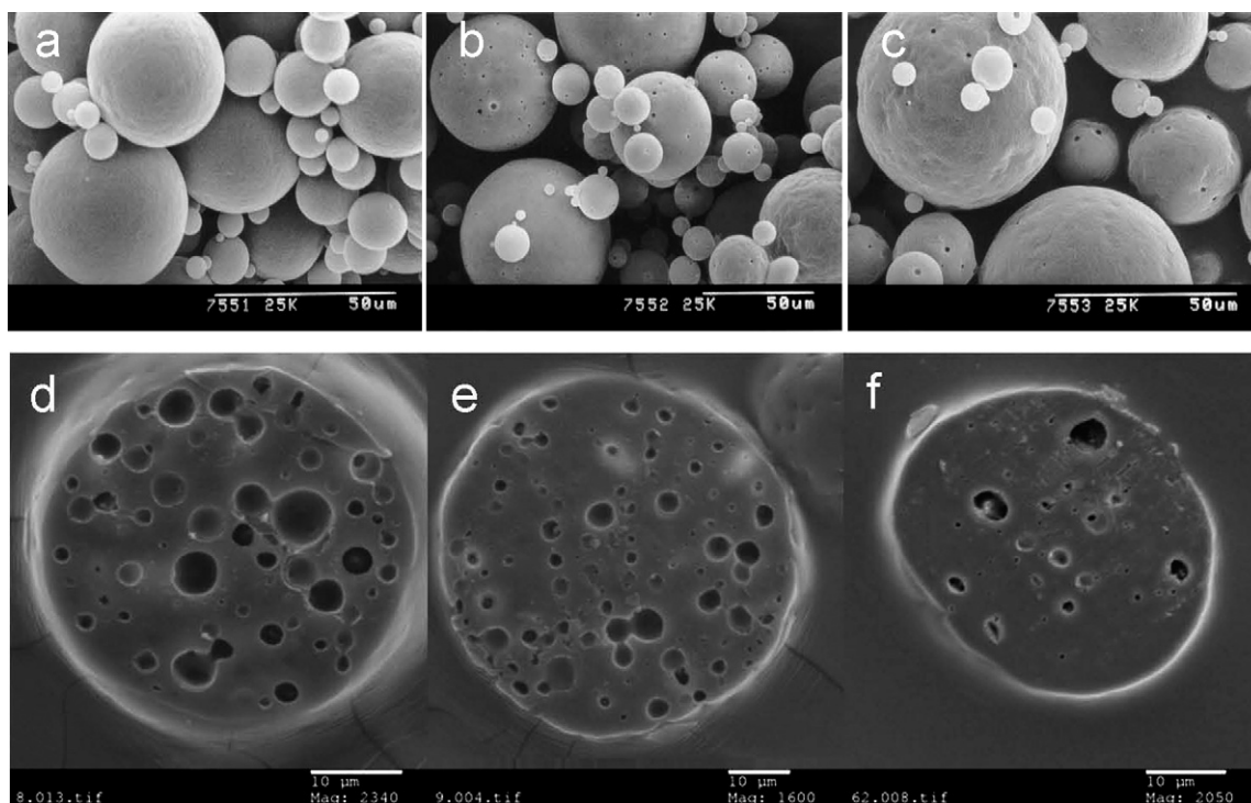
Fig. 2. Surface and internal morphology of microspheres prepared at continuous phase volume 100 ml (a, d), 200 ml (b, e) and 400 ml (c, f).
