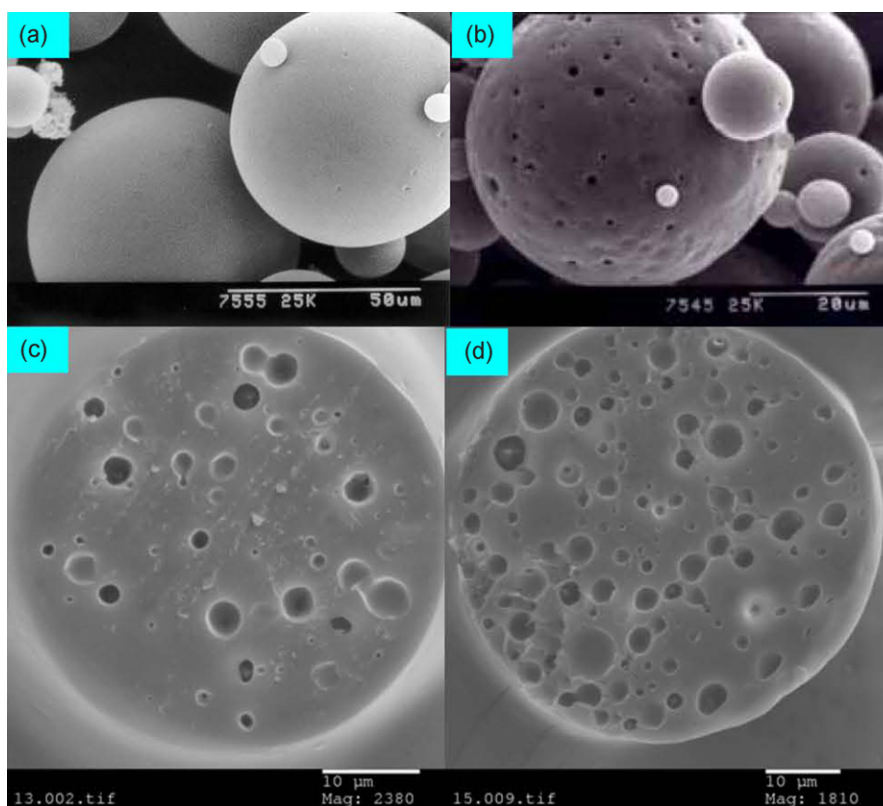
Fig. 7. Surface and internal morphology of microspheres prepared with O/W single emulsion method (a and c) and W/O/W double emulsion method (b and d).
